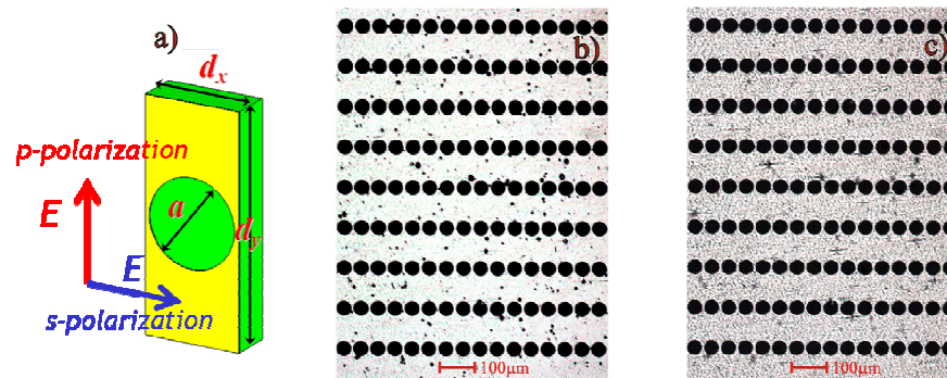
Fig. 2. (a): Geometry of hole array unit cell. Note that the PP is not perforated (b, c): Microscope images of 20 \mu m-PP-film-backed hole arrays (prototype #3) illustrating inherent granularity (surface roughness) of low-cost commercial PP-films. The case (b) corresponds to focusing on the nearest PP surface, the case (c) – focusing on the top of microhillocks.
