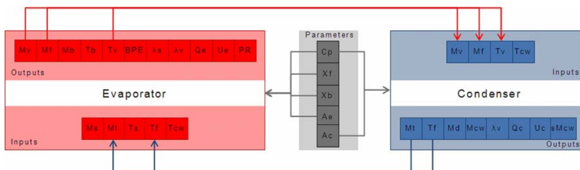
Fig. 3. Connections between the evaporator and condenser in the SEE system in TRNSYS.
