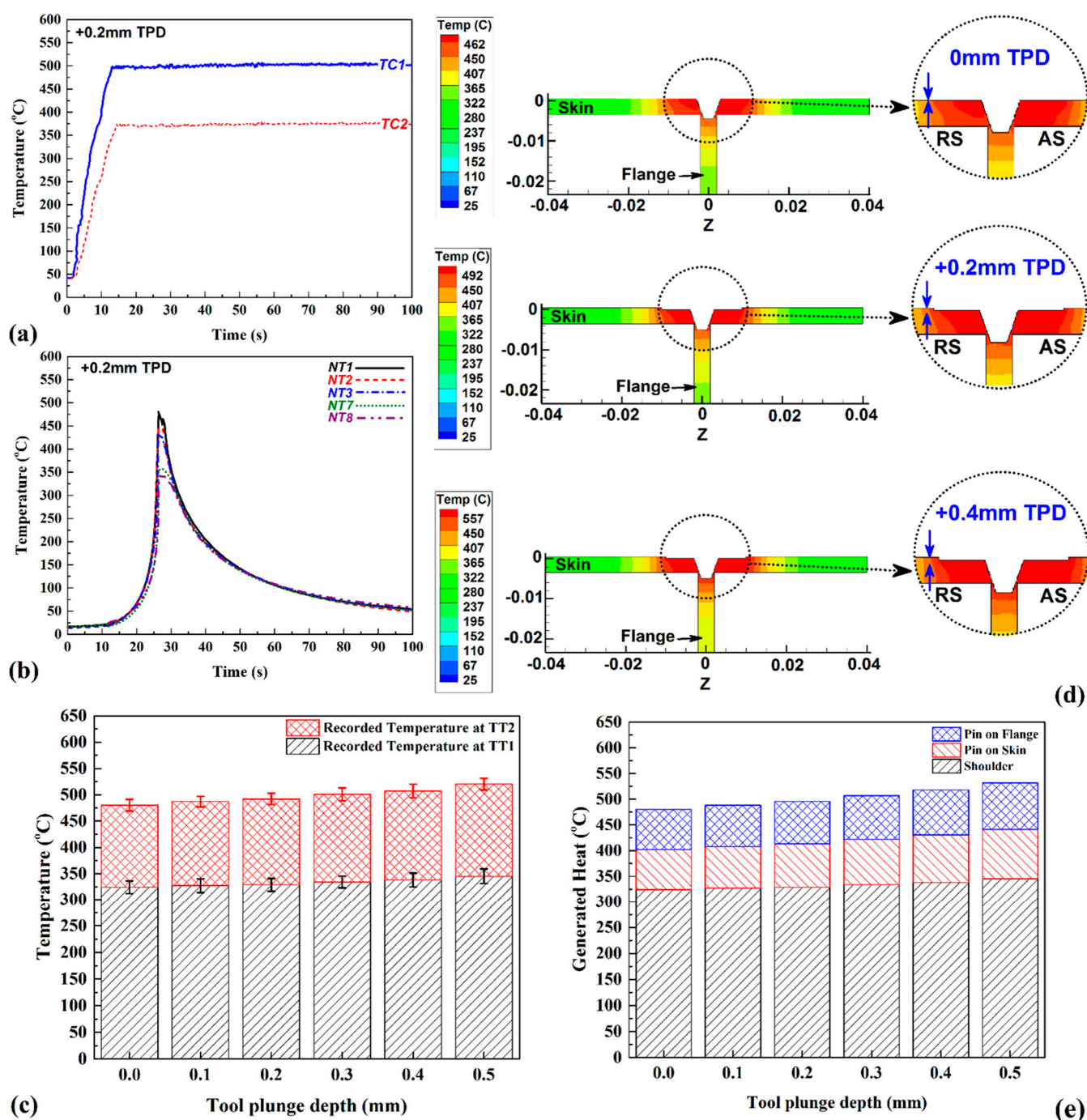
Figure 3. (a) Recorded temperature inside the FSW tool. (b) Recorded surface temperature of the joint. (c) Recorded temperature inside the FSW tool at various TPDs. (d) Cross-sectional view of the simulation results of internal heat flow. (e) Simulation results of generated heat at various TPDs.
