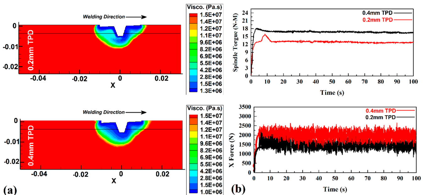
Figure 5. (a) Simulation results of internal viscosity changes at 0.2 mm and 0.4 mm TPD. (b) Force analysis of the FSW tool at 0.2 mm and 0.4 mm.
