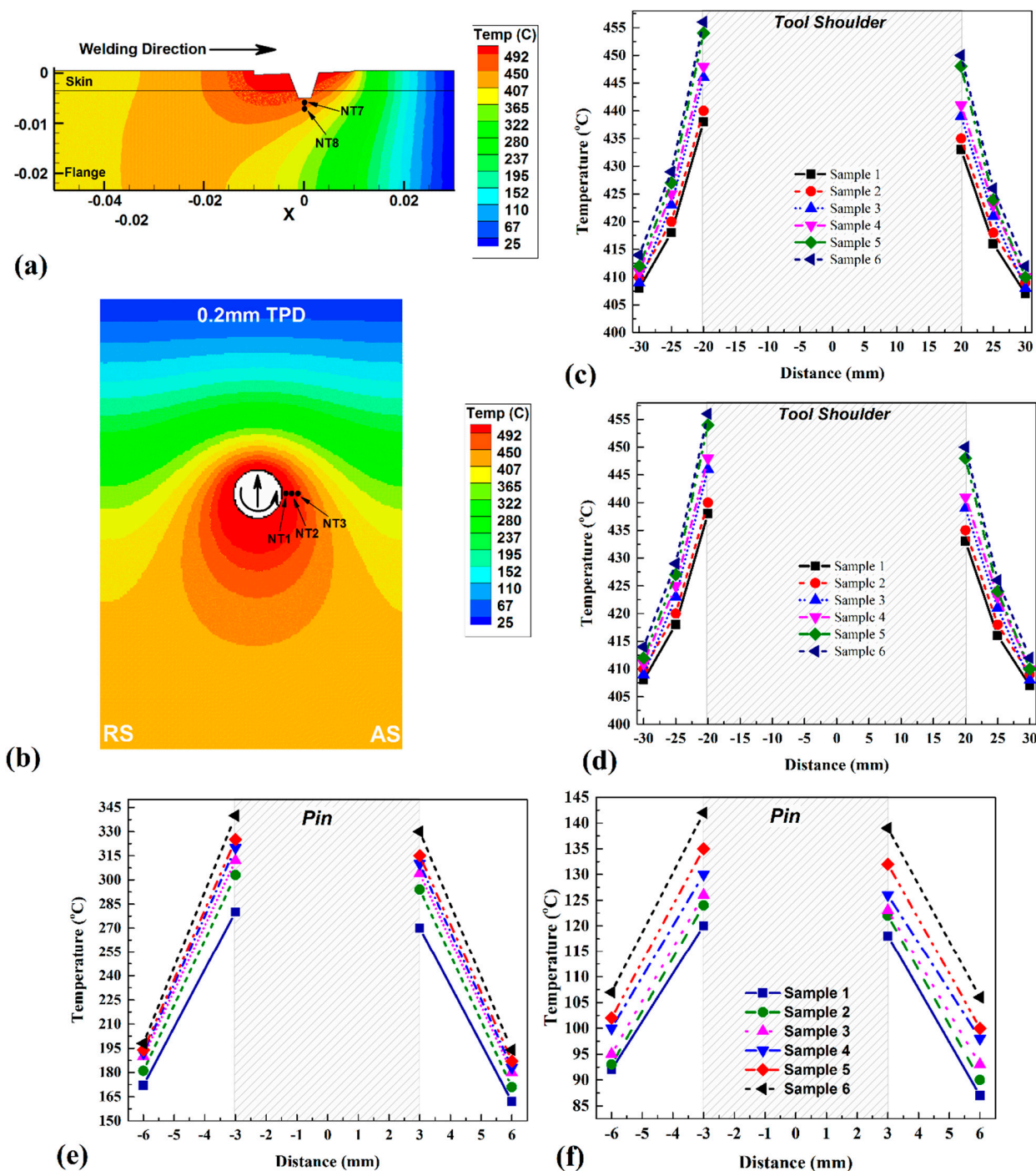
Figure 4. (a) Simulation results of internal heat flow at 0.2 mm TPD. (b) Simulation results of internal heat flow at 0.2 mm TPD. (c) Experimental and (d) maximum simulated temperature and heat diffusion on skin. (e) Recorded and (f) simulated results of maximum temperature and heat diffusion on flange.
