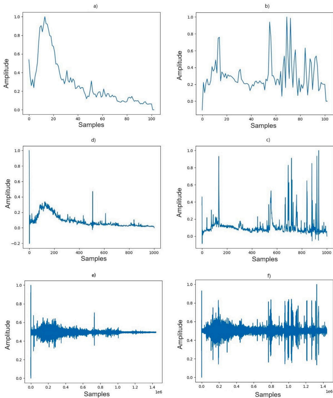
Fig. 2. (a) Envelope of a non-obstructed volunteer decimated and truncated to 100 samples. (b) Envelope of an obstructed volunteer decimated and truncated to 100 samples. (c) Envelope of an obstructed volunteer decimated and truncated to 1000 samples. (d) Envelope of a non-obstructed volunteer decimated and truncated to 1000 samples. (e) Original signal of a non-obstructed volunteer more than 1.4 million samples. (f) Original signal of an obstructed volunteer more than 1.4 million samples. For more information, see https://github.com/mario42004/urossound .
