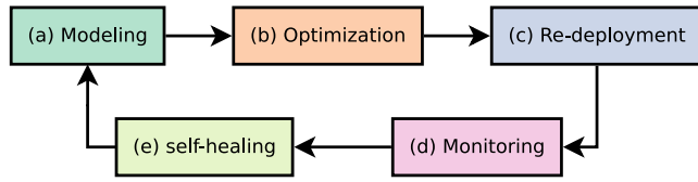
Figure 2: The application lifecycle supported by the IEM.
