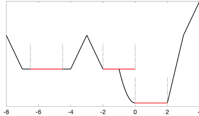
Fig. 2. An example of function satisfying u_T \in \mathcal{R}_T for the Hamiltonian H(p) = |p| and T = 1 . In view of Corollary 2, we only need to check the interior ball condition at the local minima of u_T . For each local minimum x of u_T in this plot, we have colored in red a ball of radius 1 around x , in which u_T is smaller or equal than u_T(x) .
