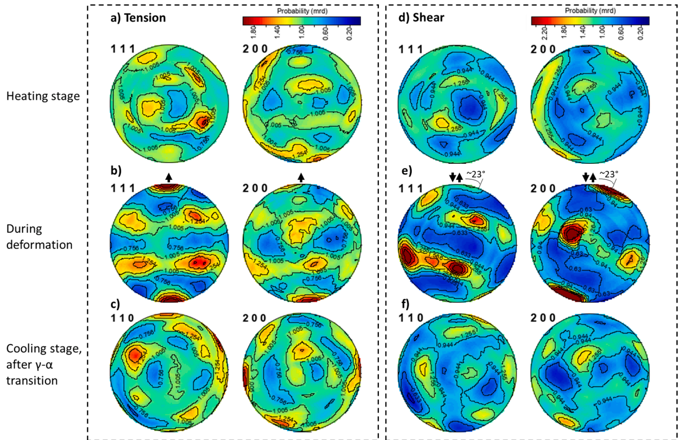
Fig. 7. Pole figures (top) before, (middle) during and (bottom) after the (a-c) tensile and (d-f) shear deformation experiments on 44MnSiV6 at 1300 °C and 1330 °C, respectively. The load direction is vertical (black arrows). The initially untextured samples show preferred orientations during deformation, which dissipate again during cooling and the \gamma - \alpha phase transition.
