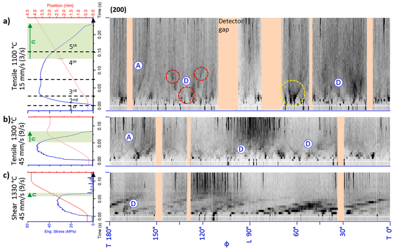
Fig. 6. Diffraction intensity evolution of the (200) ring along 180° of the azimuth over time during (a) the tensile deformation at 1100 °C and 3 s -1 , E1, (b) the tensile deformation at 1300 °C and 9 s -1 , E2, (c) the shear deformation at 1330 °C and 9 s -1 , E3. Time progresses from bottom to top in each plot whilst a darker colour indicates a higher intensity. Regions with DRX 'islands' are annotated with (D), arcs with varying intensity as (A). The white blocks remain from gaps in the detector, as seen in Fig. 4(a–f), and are marked with orange blocks for clarity. The change of macro-stress (blue) and position (red) during each experiment are shown on the left for comparison.
