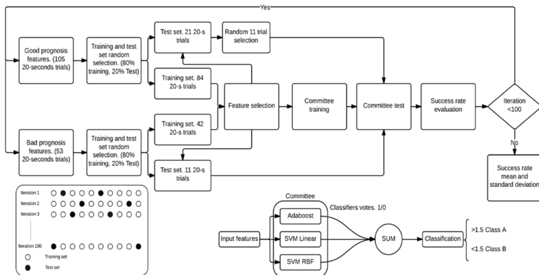
Fig. 1. Classification architecture.
